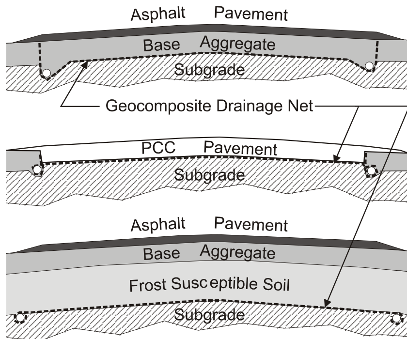
Figure 2 - Potential applications of geocomposite drainage net
