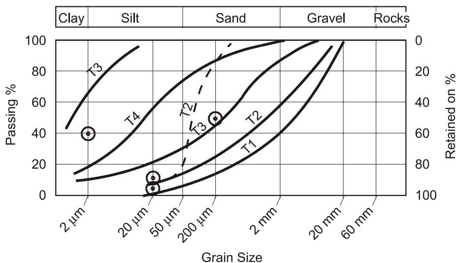
Figure 1 - Norwegian frost susceptibility criteria
